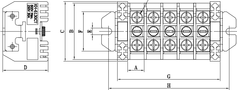
KH-6130CT-NDN
