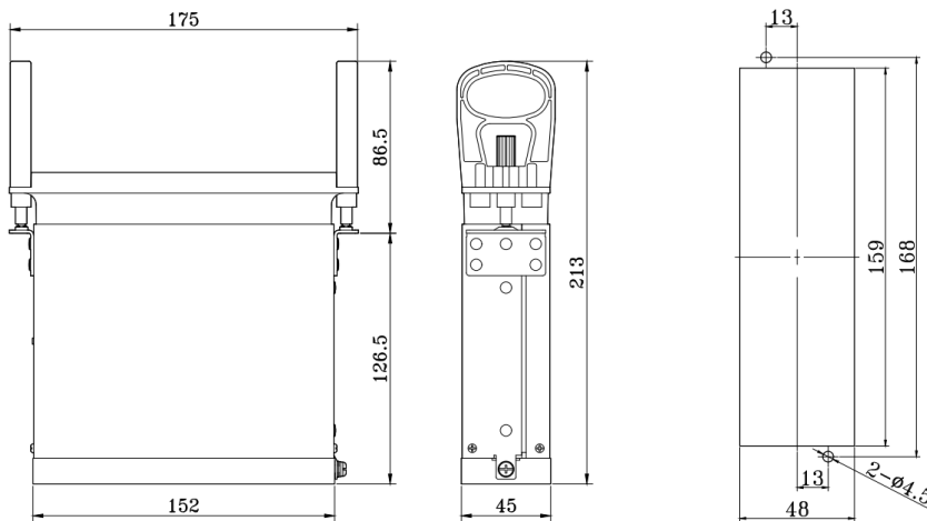
[Panel CUT-OUT]
