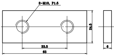
KH-60200
