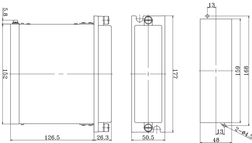
[Panel CUT-OUT]
